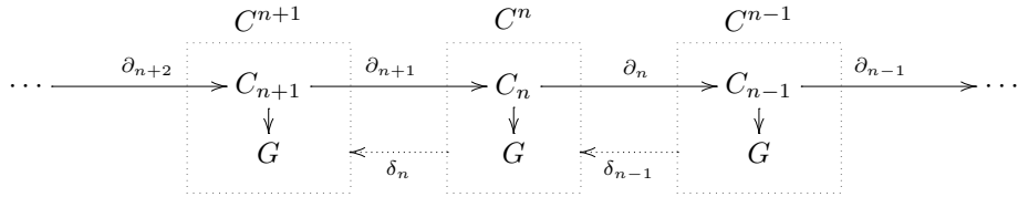
Figure 10: Structure of the cochain complex.
